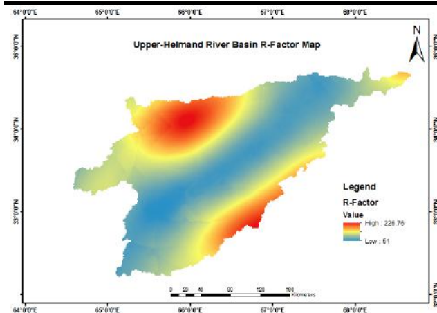
Fig.2: R-Factor Map Upper-Helmand Catchment
