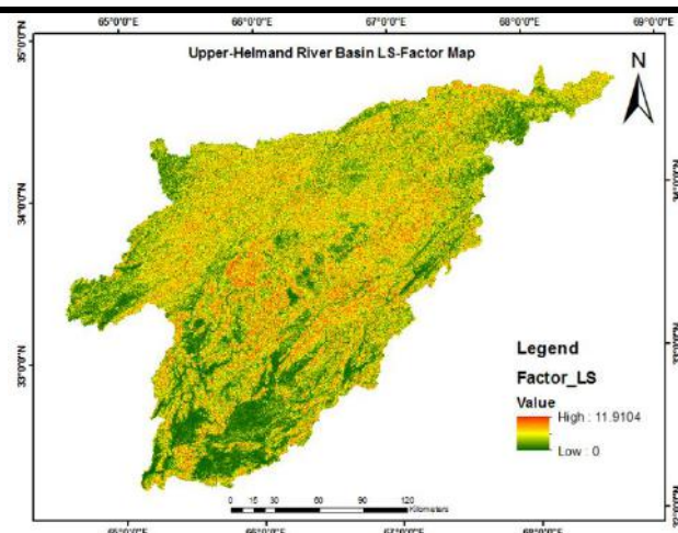
Fig.5 LS-Factor Map of Upper-Helmand Catchment
