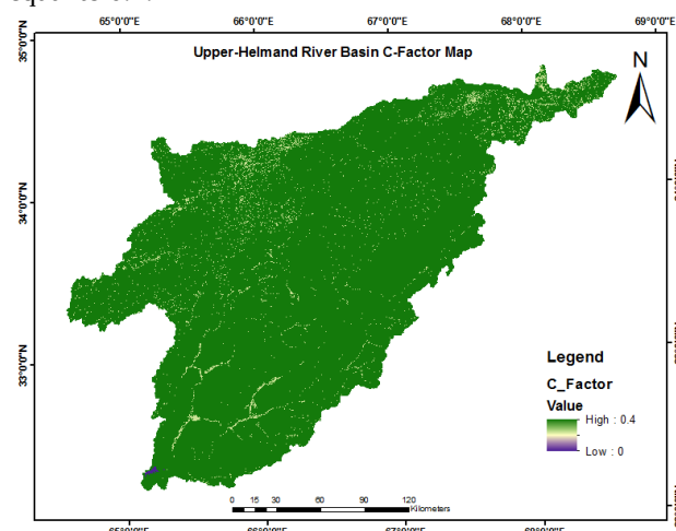
Fig.6 C_m -Factor Map of Upper-Helmand Catchment
